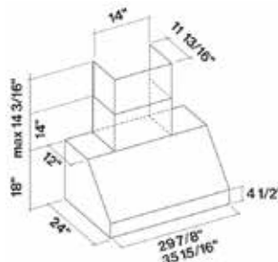
Optional Duct Cover Shown
