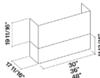
Optional Duct Cover
