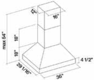
Island Mount
