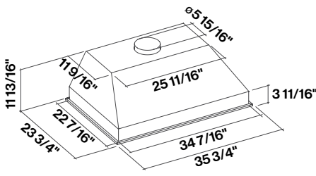
34" x 22" Depth Single Blower
