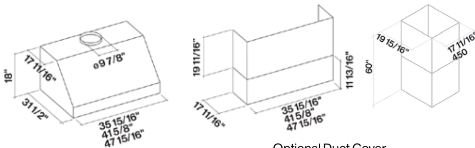
Optional Duct Cover
