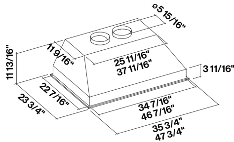
34"/46" x 22" Depth Dual Blower
