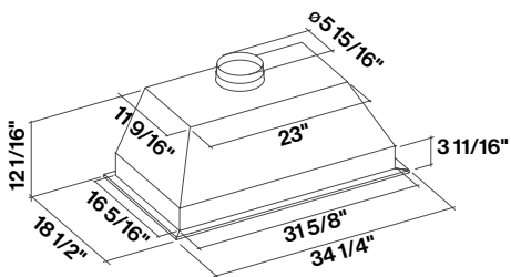
34" x 18" Depth Single Blower
