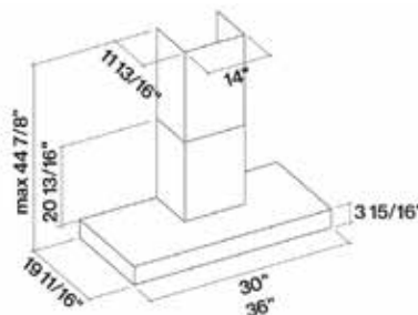
Wall Mount
