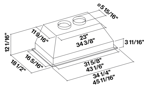
34"/46" x 18" Depth Dual Blower
